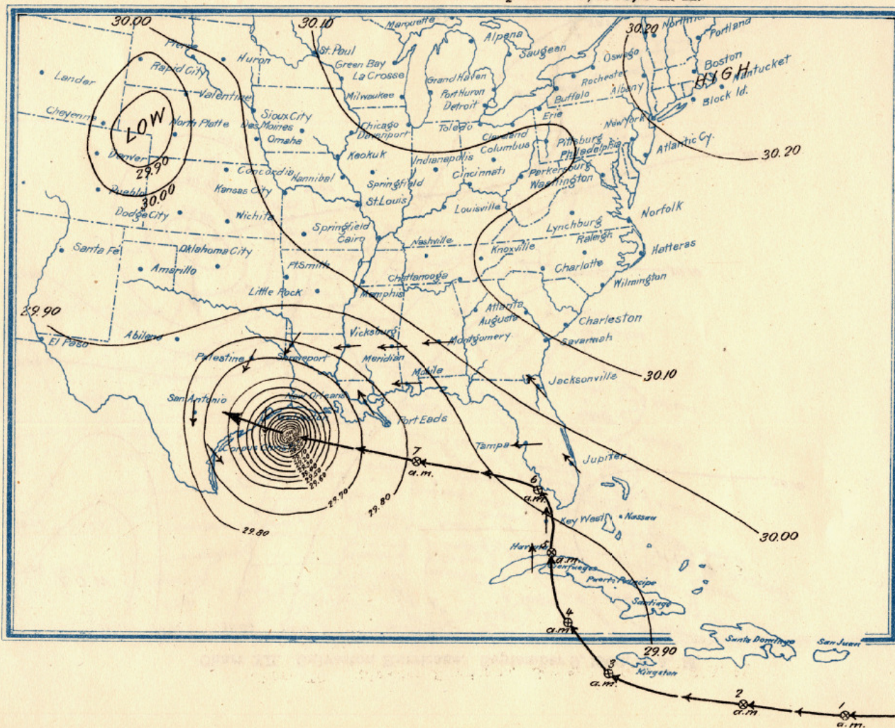
Chart XI. Galveston Hurricane. September 8, 1900, 8 A. M.
